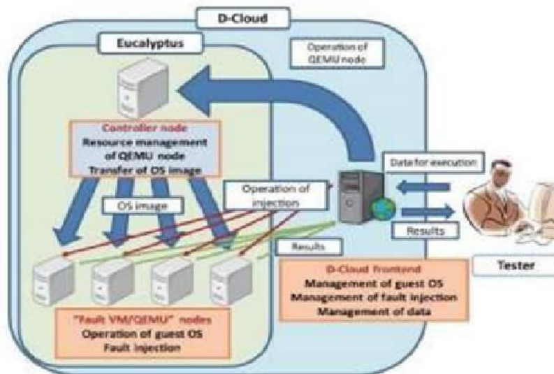
Fig. 5. Architecture of D-Cloud
